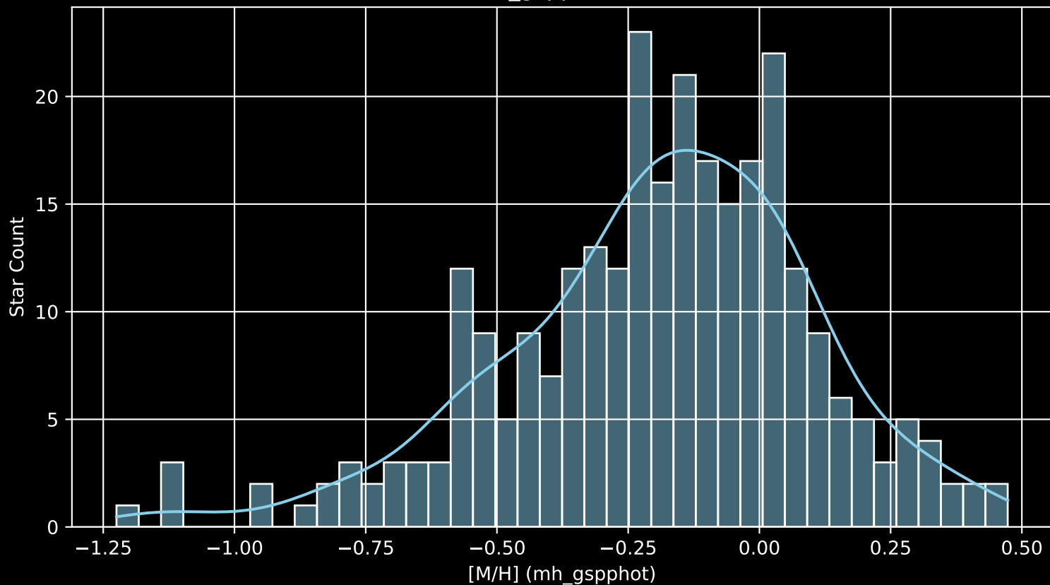
APOGEE DR17 Field: [126-24_btx [M/H] (mh_gspphot) (n= 283)
