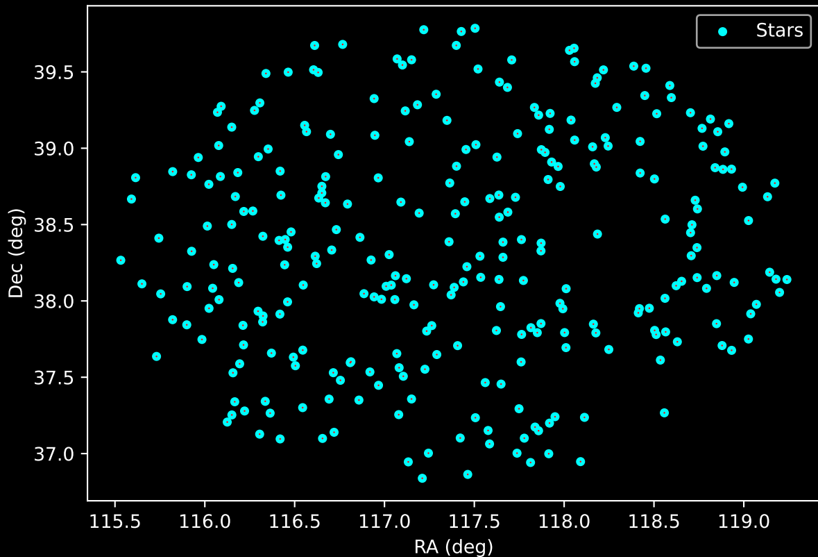
APOGEE DR17 Field: [126-24_btx] Proper Motion Vectors for Gaia Star Field (n= 286)
