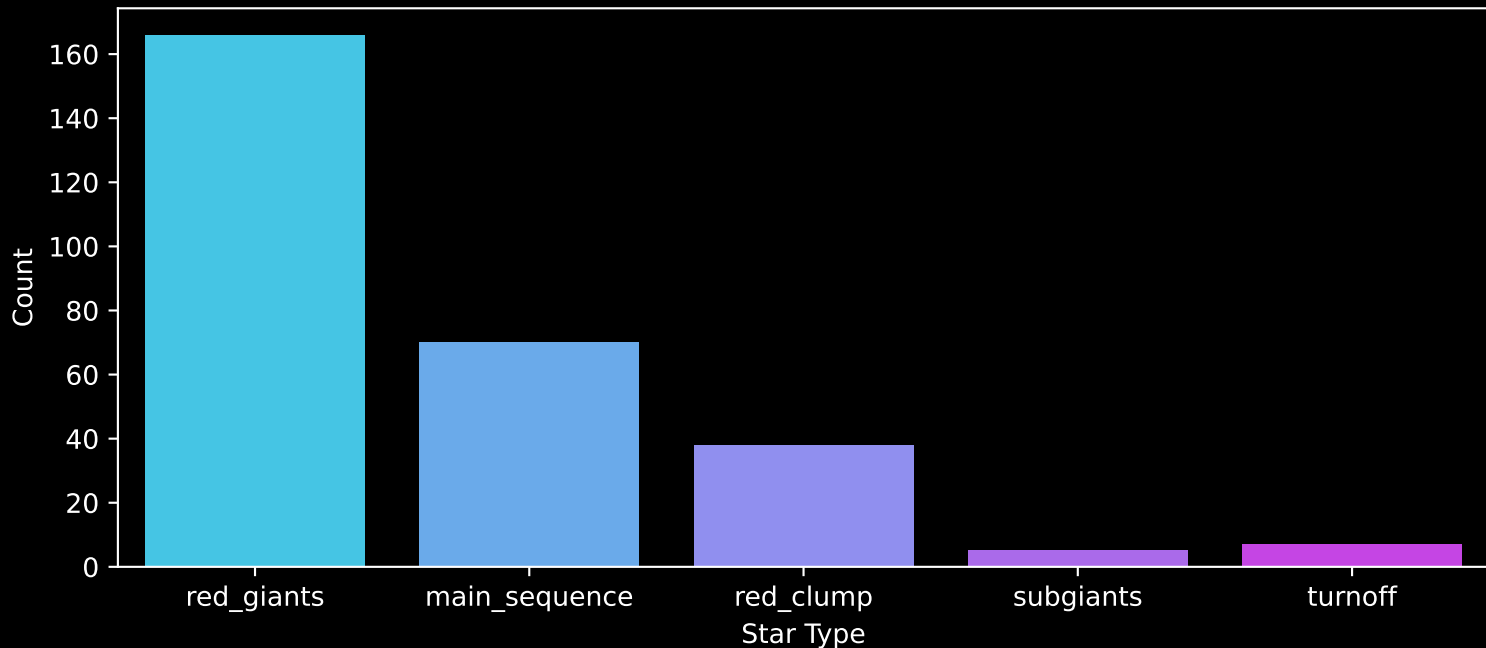
APOGEE DR17 Field: [126-24_btx] Count plot of Star Type
