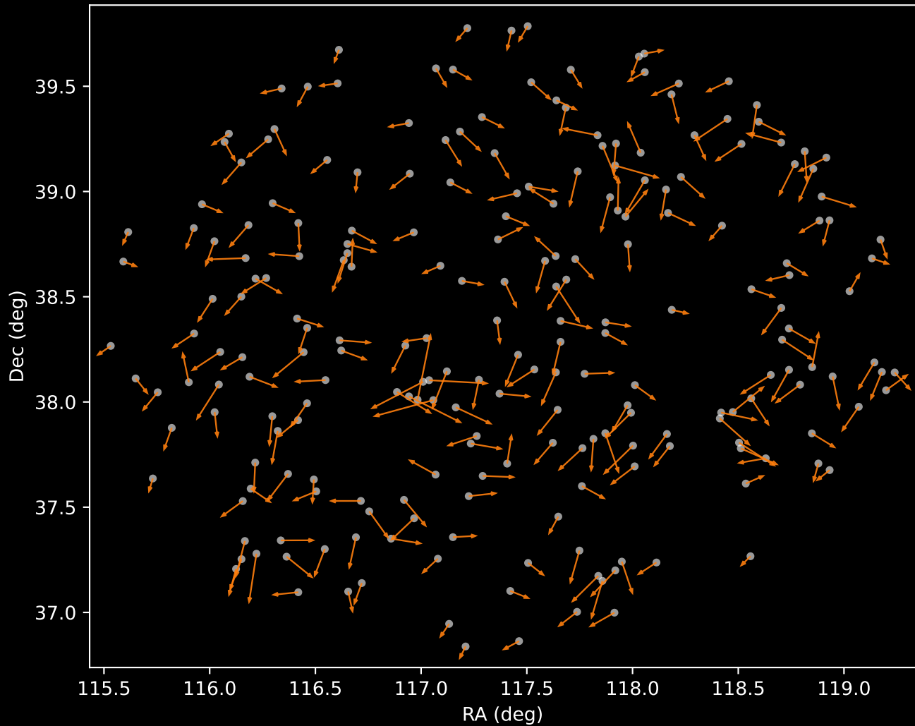
APOGEE DR17 Cluster 2 Proper Motion Vectors (n=226)
