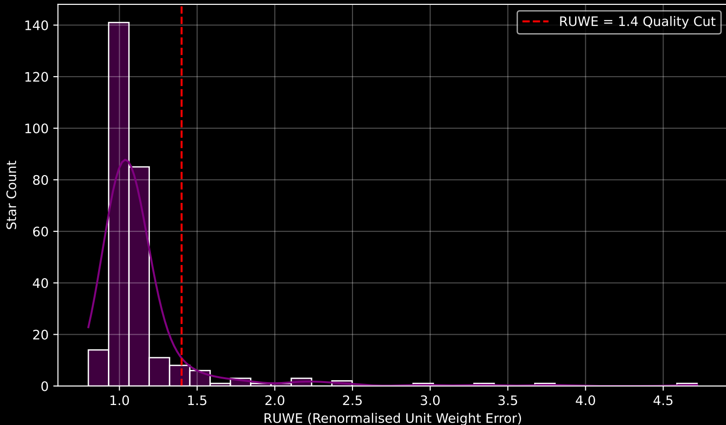
GAPOGEE DR17 Field [126-24_btx] RUWE Distribution (n= 280)
