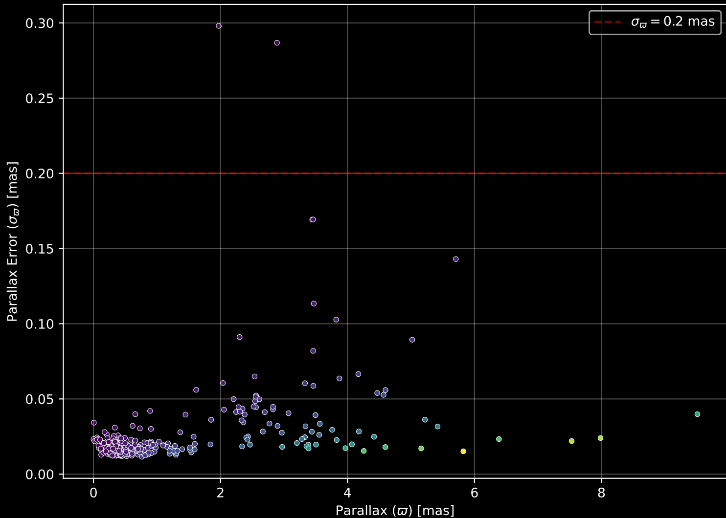
APOGEE DR17 Field: [126-24_btx] Parallax Quality (n= 286)
