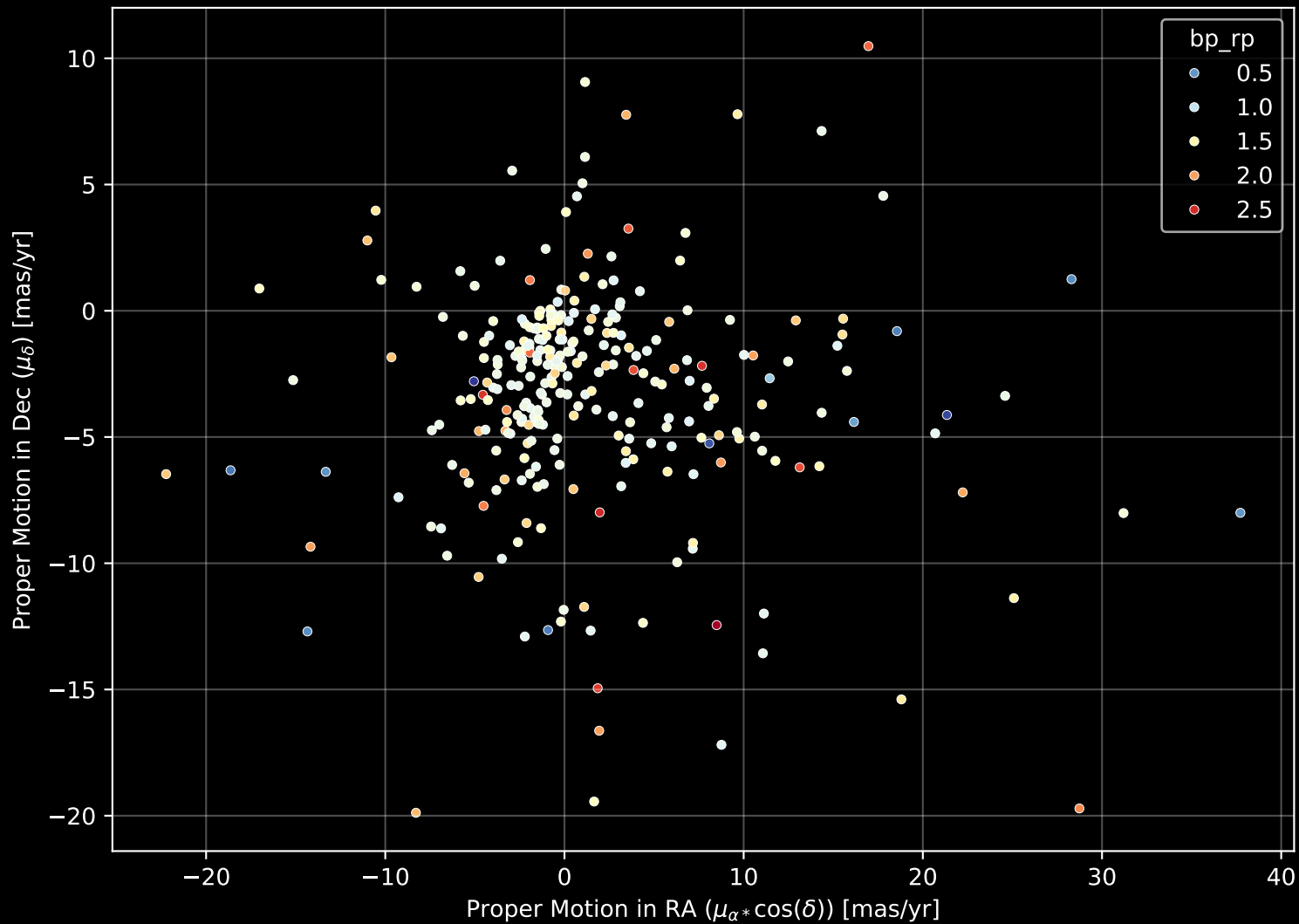
APOGEE DR17 Field: [126-24_btx] Proper Motion Diagram (n= 286)
